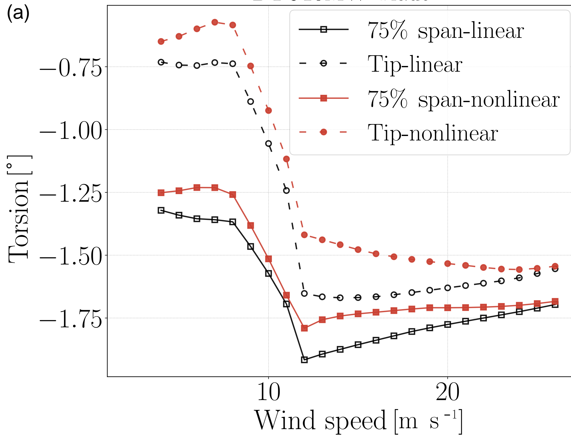
DTU10MW blade
