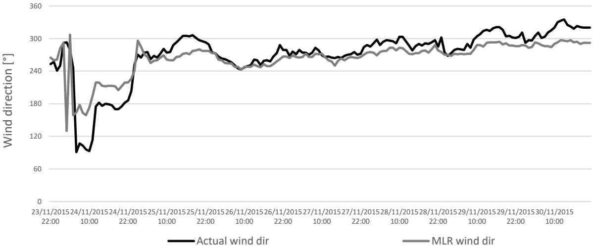
Wind direction - actual and predicted using MLR MCP methodology
