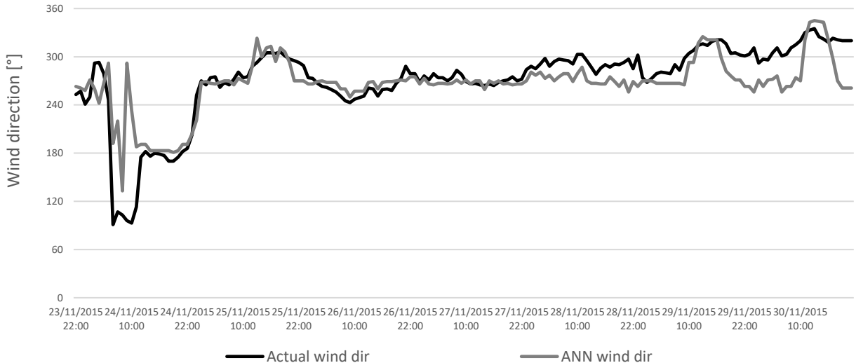
Wind direction - actual and predicted using ANN MCP methodology
