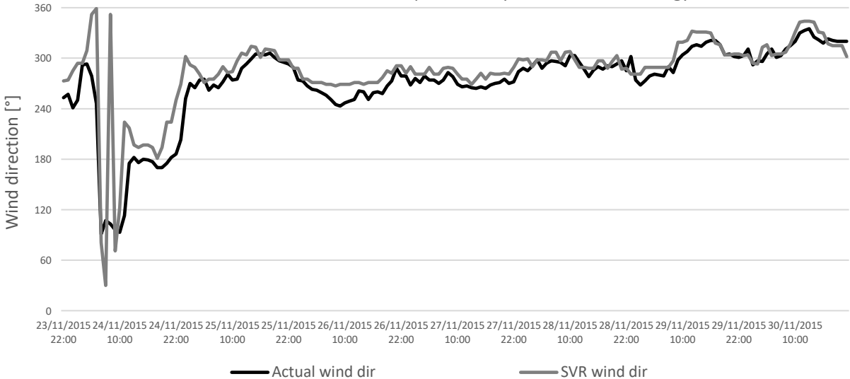
Wind direction - actual and predicted by SVR MCP methodology
