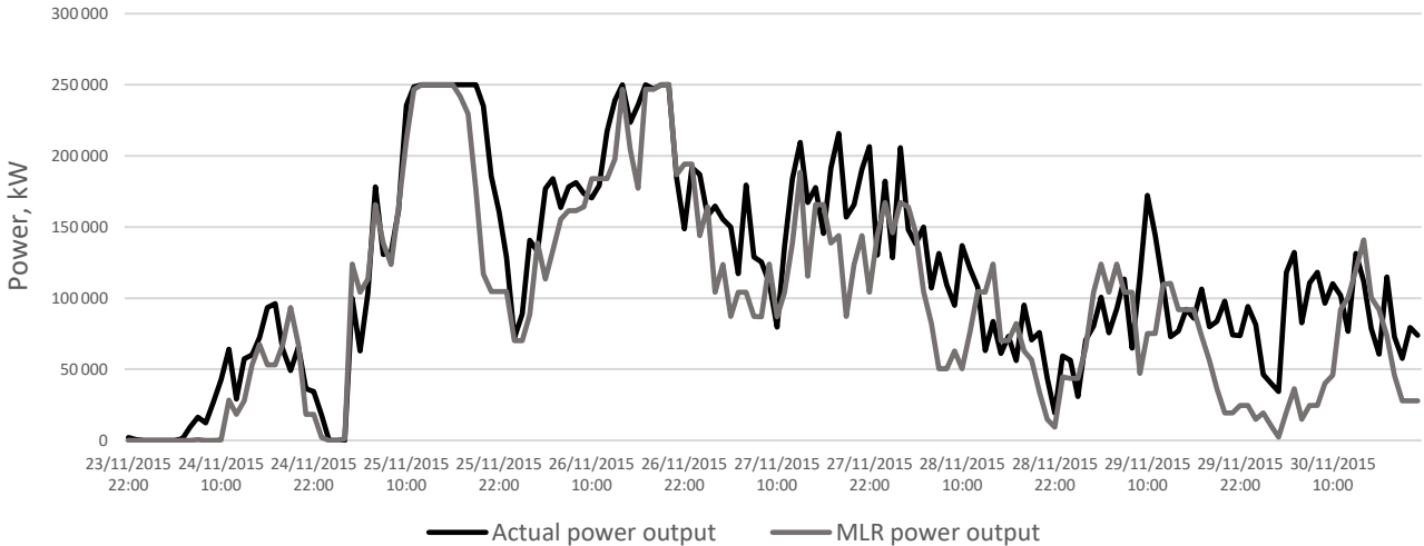
Wind farm power output, kW - actual and predicted by MLR MCP methodology
