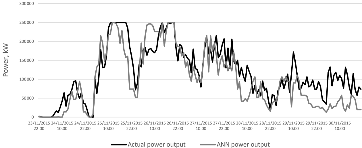
Wind farm power output, kW - actual and predicted by ANN MCP methodology
