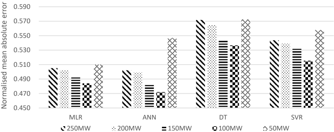
Normalised mean absolute error
