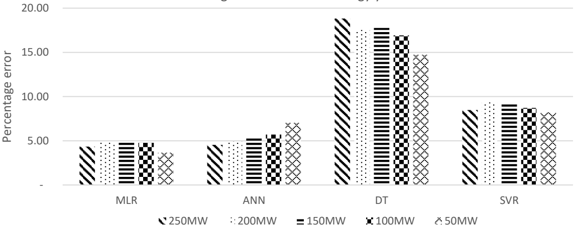
Percentage error in overall energy yield
