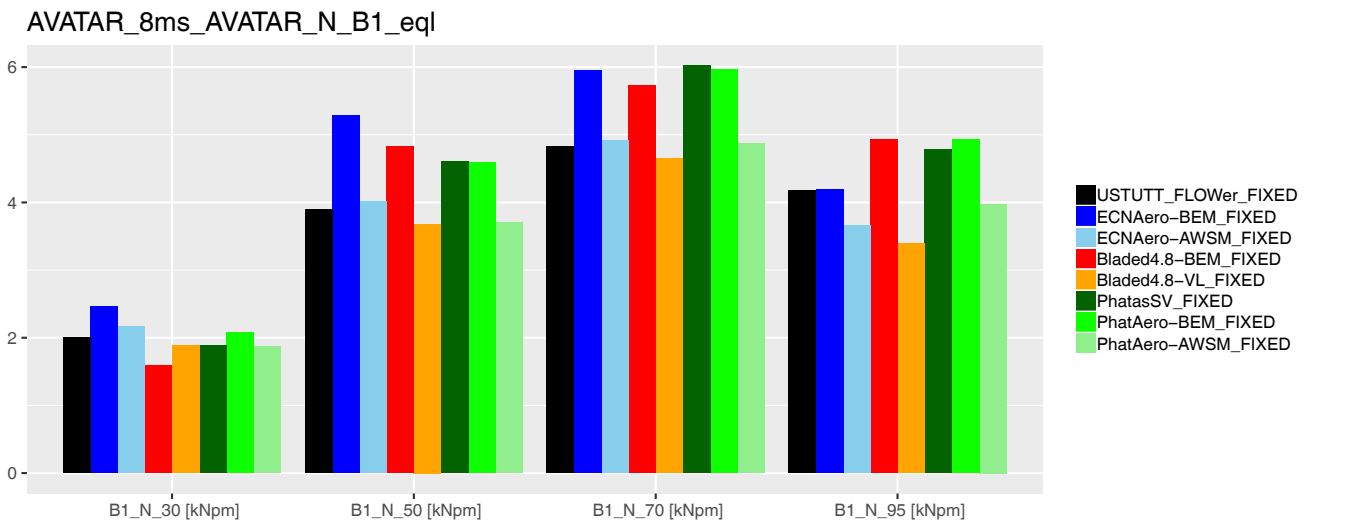
(b) Fatigue equivalent of chord normal force at 30%R, 50%R, 70%R and 95%R
