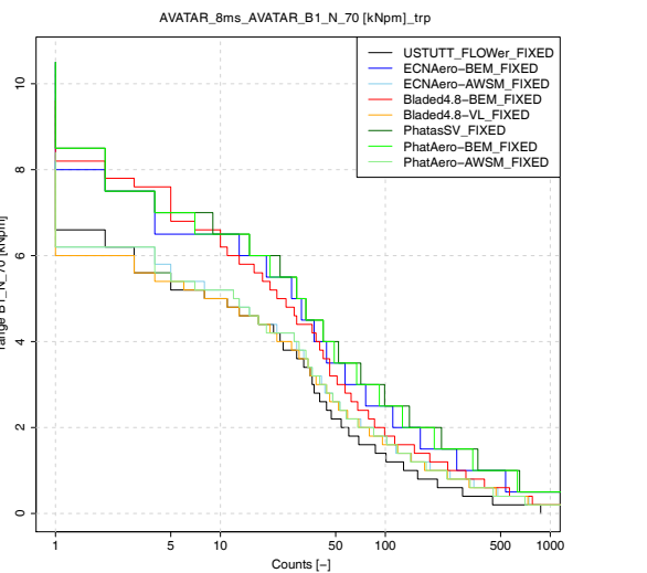
(c) Staircase plot of chord normal force at 70%R
