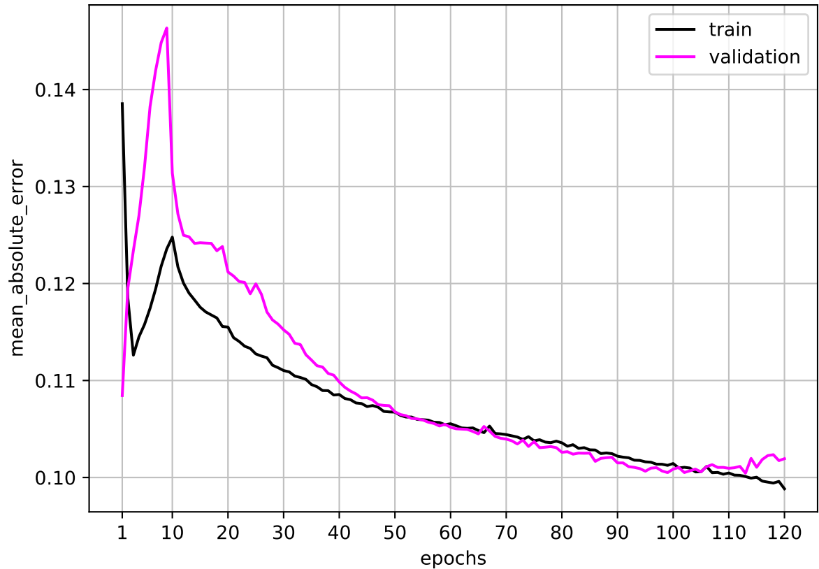
LSTM Training History, mean_WS = 7m/s, TI = 10%, lag = 30s
