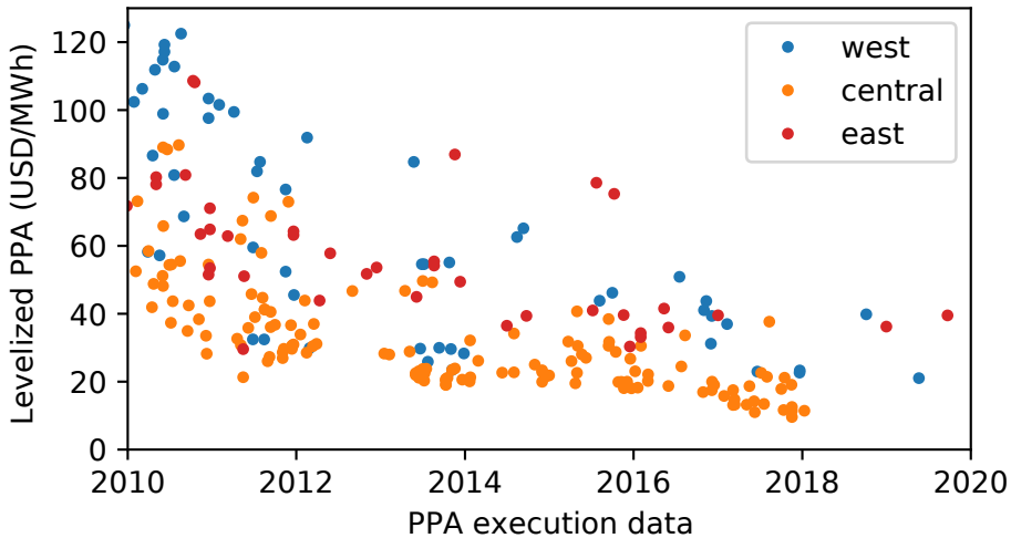
PPAs of U.S. Wind Farms since 2010
