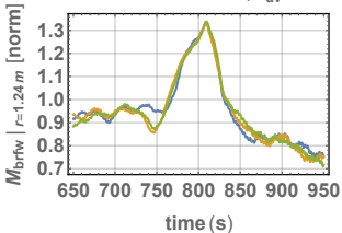
stand-alone: case 5, \tau_{av}=20 s
