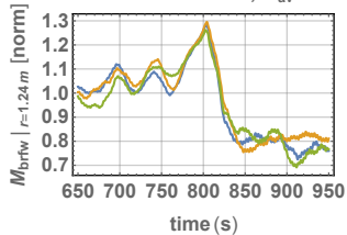
stand-alone: case 3, \tau_{av}=20 s
