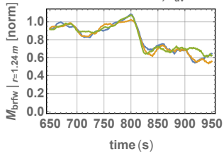
stand-alone: case 2, \tau_{av}=20 s
