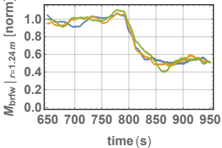
stand-alone: case 1, \tau_{av}=20 s
