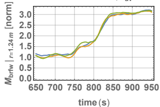
stand-alone: case 7, \tau_{av}=20 s
