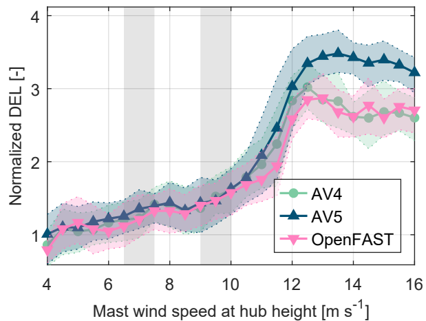
(c) Tower-base fore-aft bending moment
