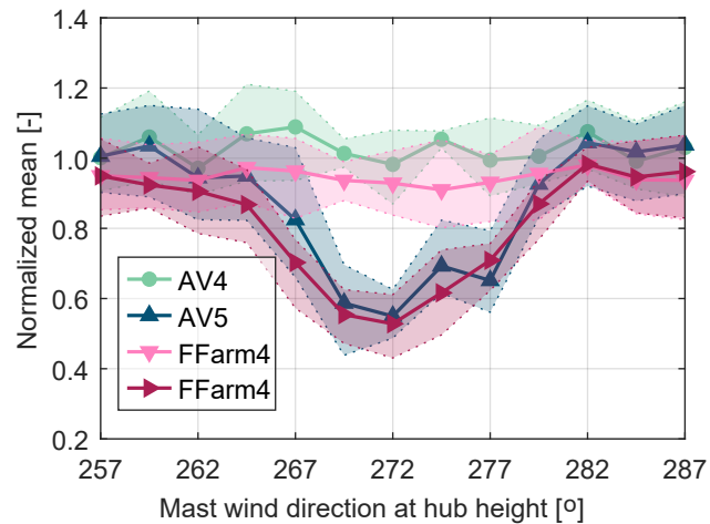
(c) Wind speed bin II (9.0 – 10.0 m s -1 )
