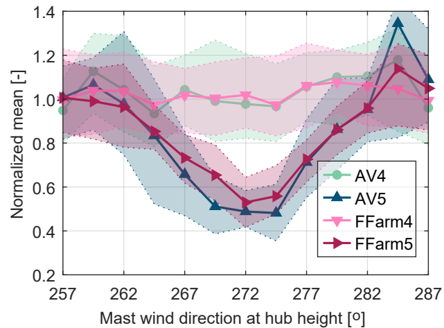
(a) Wind speed bin I (6.5 – 7.5 m s -1 )
