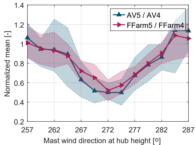
(b) Wind speed bin I (6.5 – 7.5 m s -1 ) normalized by freestream values
