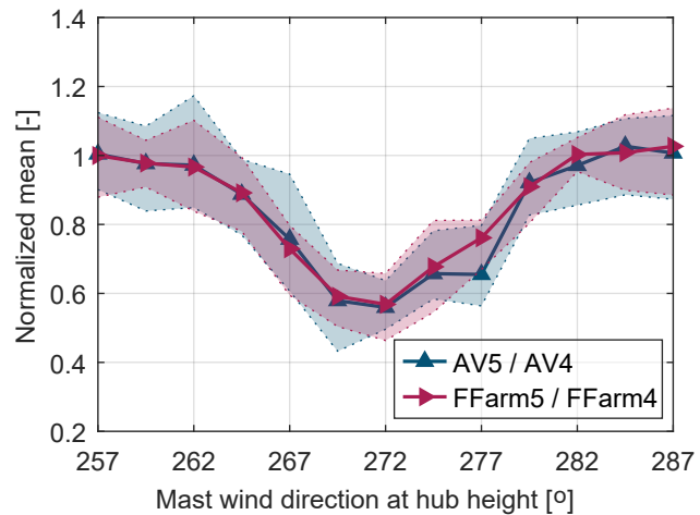
(d) Wind speed bin II (9.0 – 10.0 m s -1 ) normalized by freestream values
