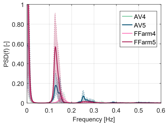
(a) Blade-root flapwise bending moment
