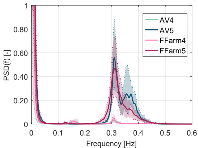
(b) Tower-base fore-aft bending moment
