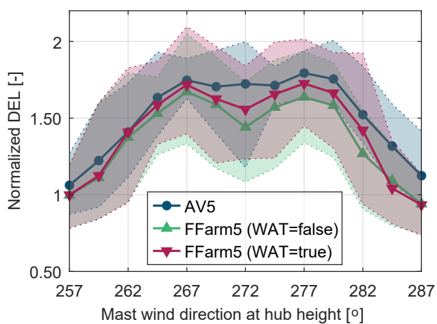
(a) Blade-root bending moment in flapwise direction
