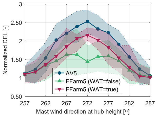
(b) Tower-base bending moment in fore-aft direction
