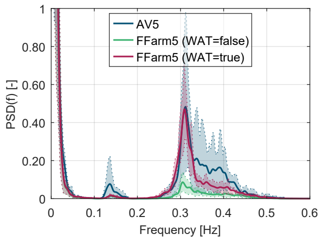
(b) Tower-base fore-aft bending moment
