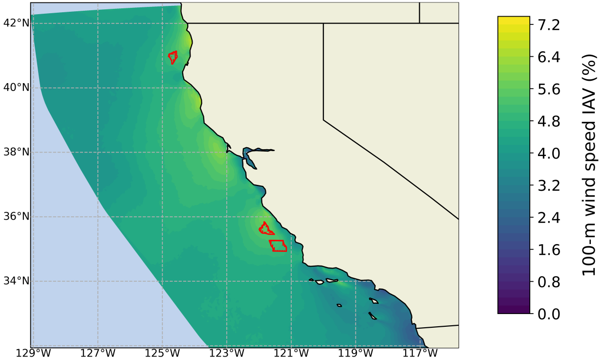
Figure S1: Interannual variability in 100-m wind speed calculated using the WRF 20-year data.
