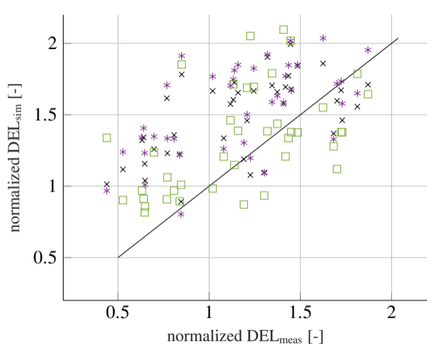
Tower bottom fore-aft moment (m=4)
