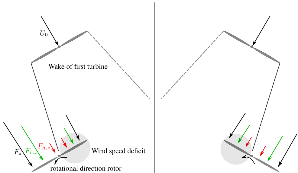
Flapwise blade root bending moment
