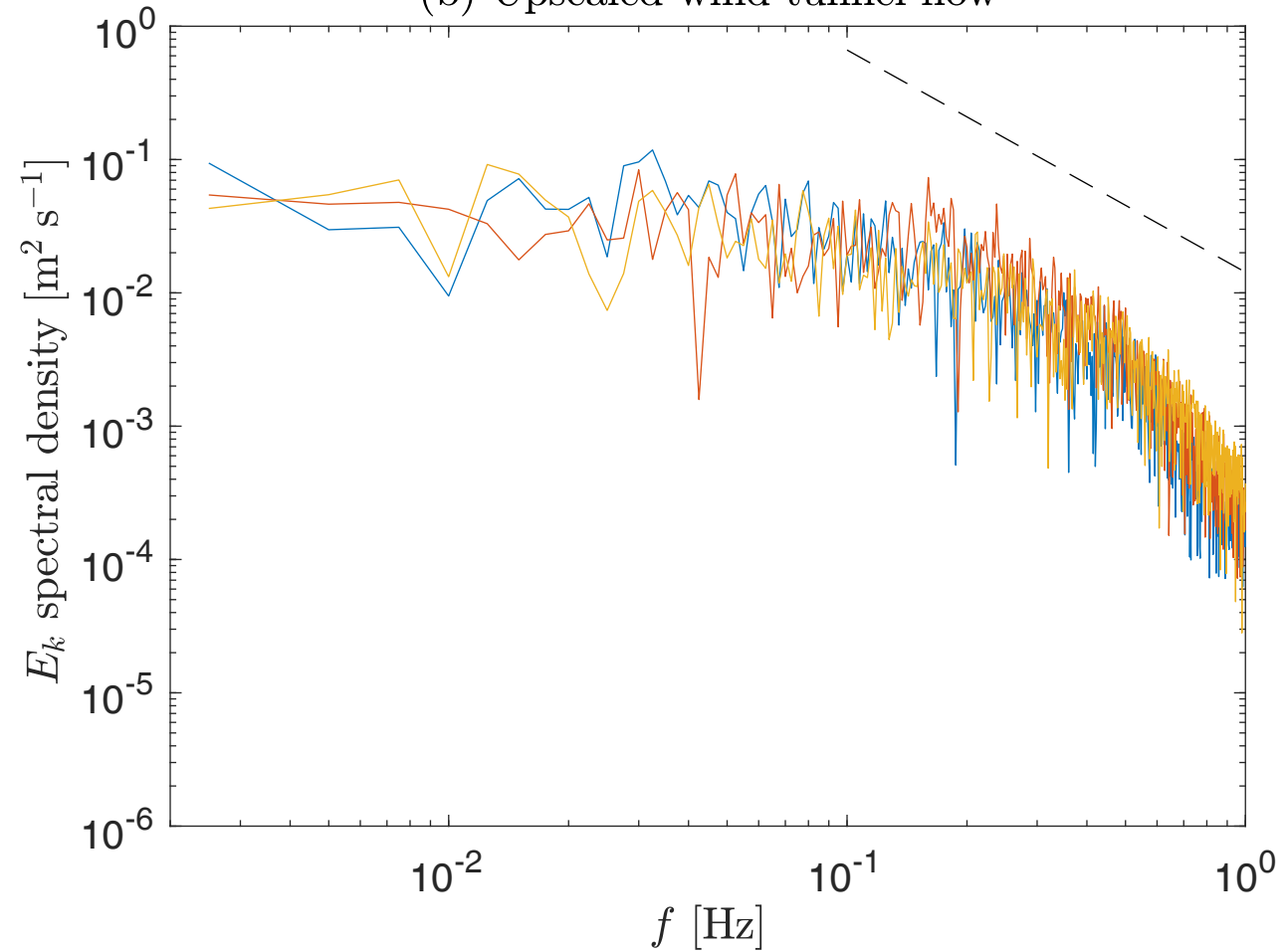
(b) Upscaled wind tunnel flow
