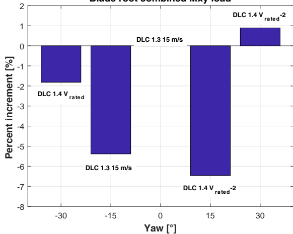
Blade root combined Mxy load
