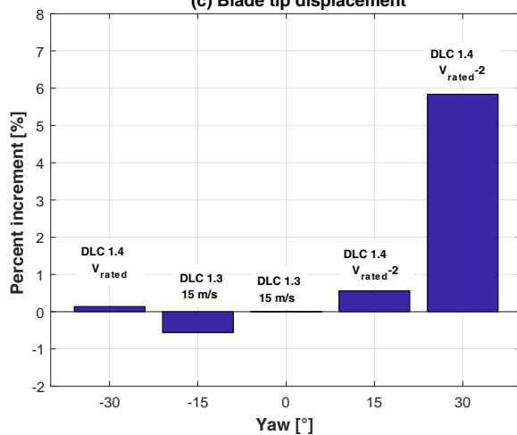
(c) Blade tip displacement
