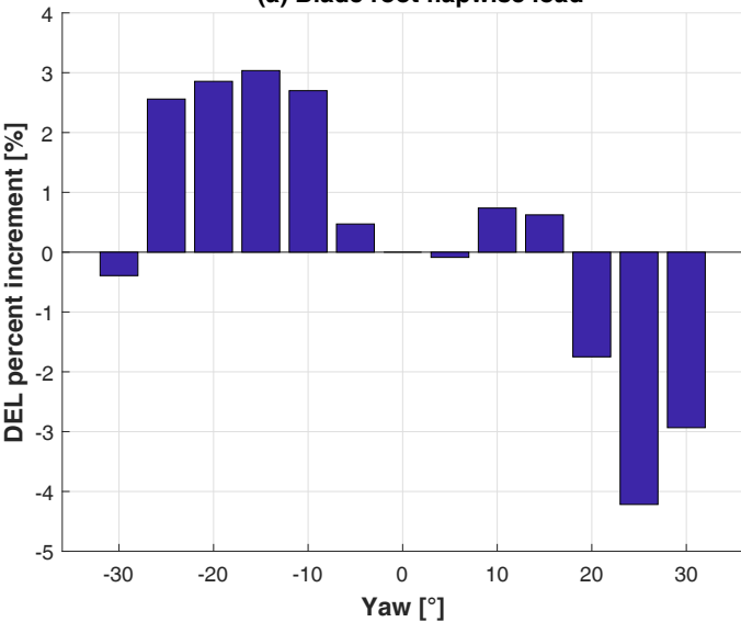
(a) Blade root flapwise load
