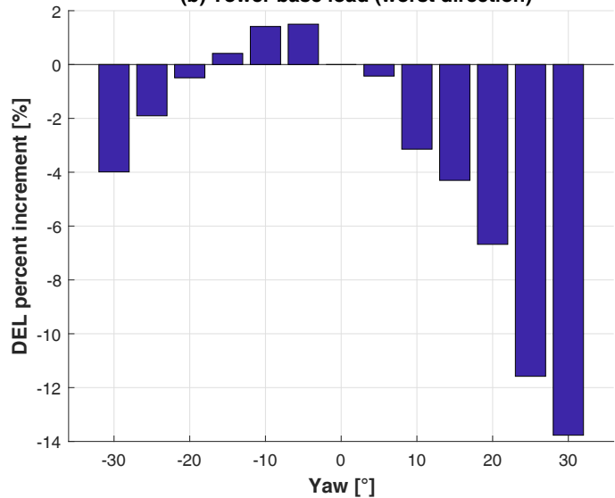
(b) Tower base load (worst direction)
