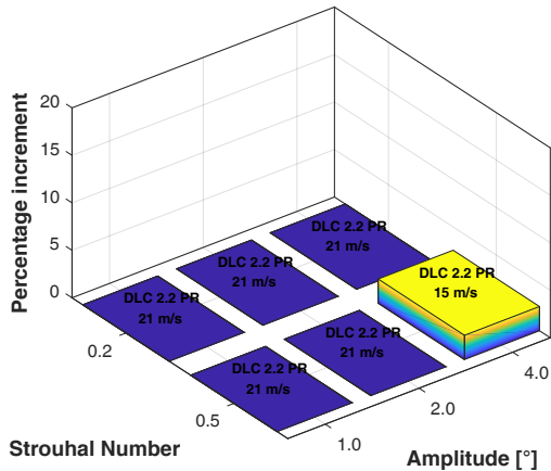
(c) Ultimate load Hub fixed combined load
