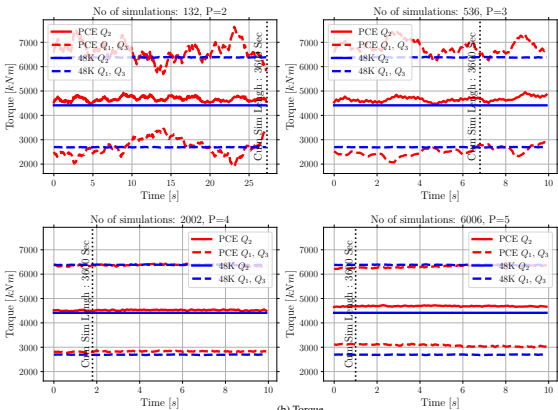
(b) Torque
