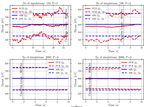
(a) Thrust
