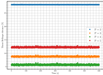
(a) Thrust
