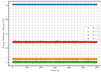
(b) Torque
