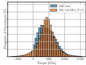
(b) Torque
