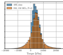
(b) Torque
