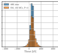
(a) Thrust
