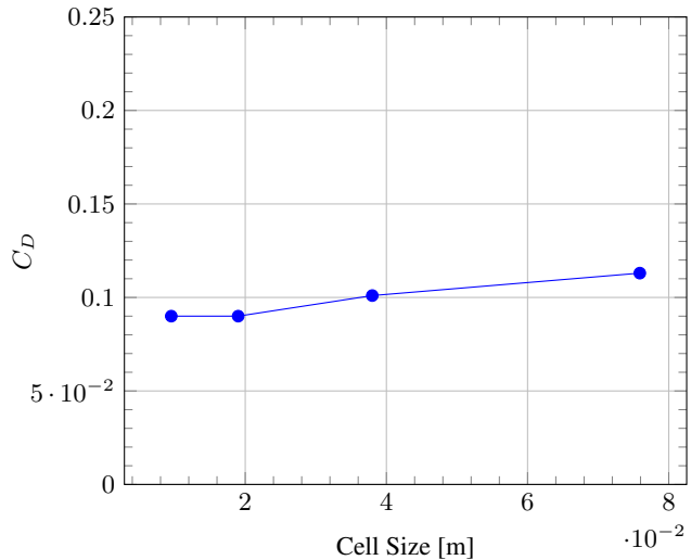
(b) Drag coefficient C_D
