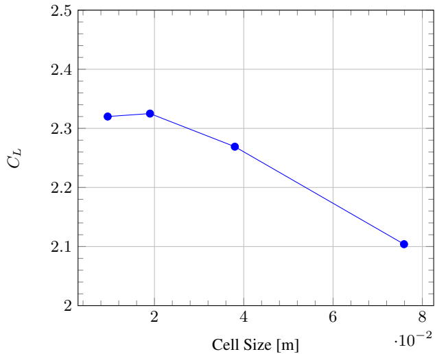
(a) Lift coefficient C_L
