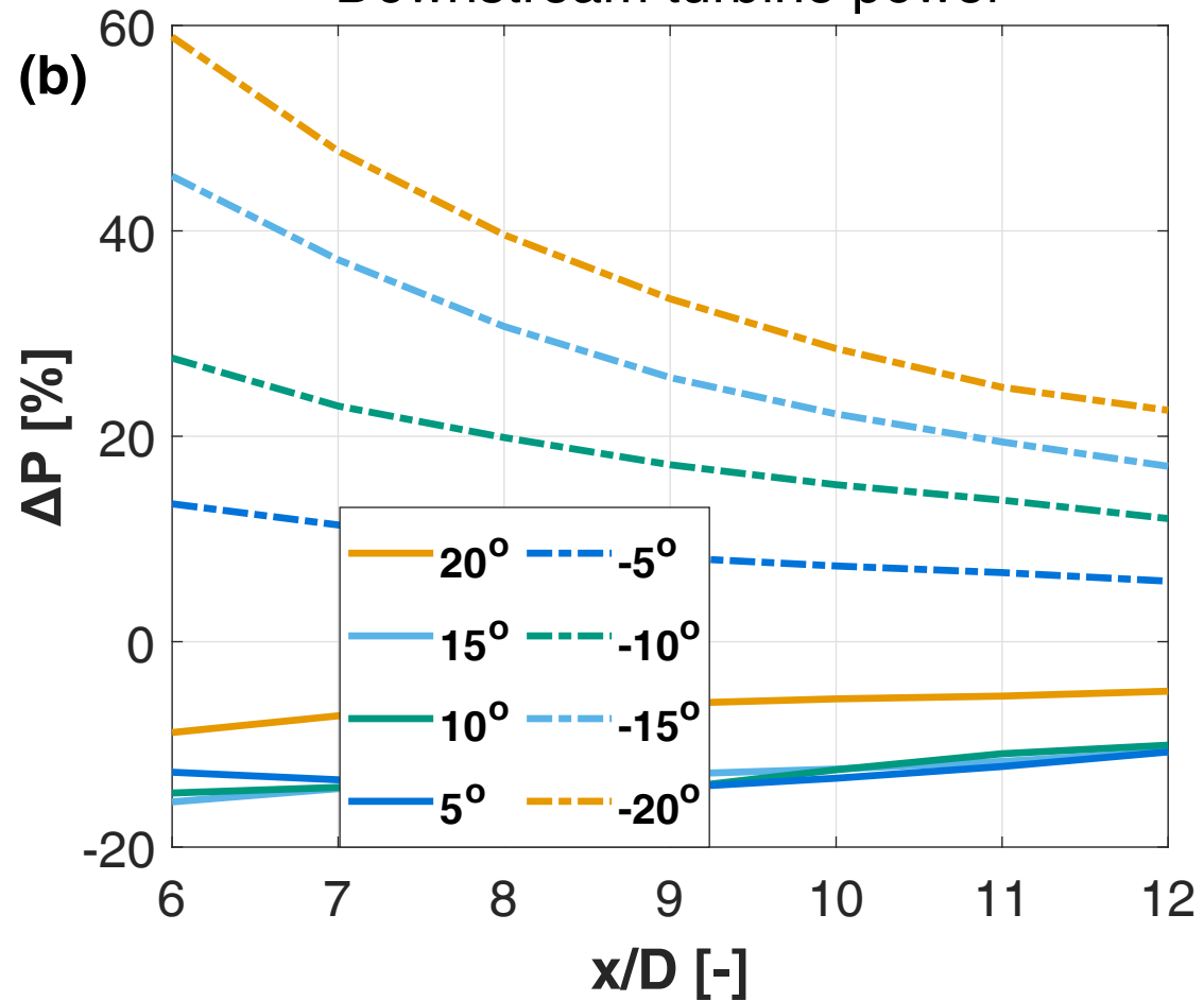
Downstream turbine power
