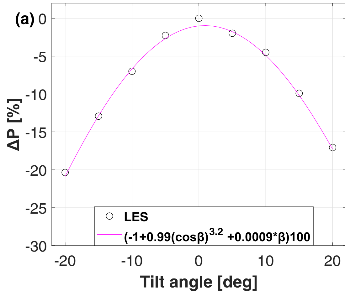
Upstream turbine power
