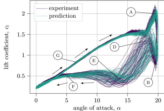
(a) Lift DTW + EMD score = 1.16
