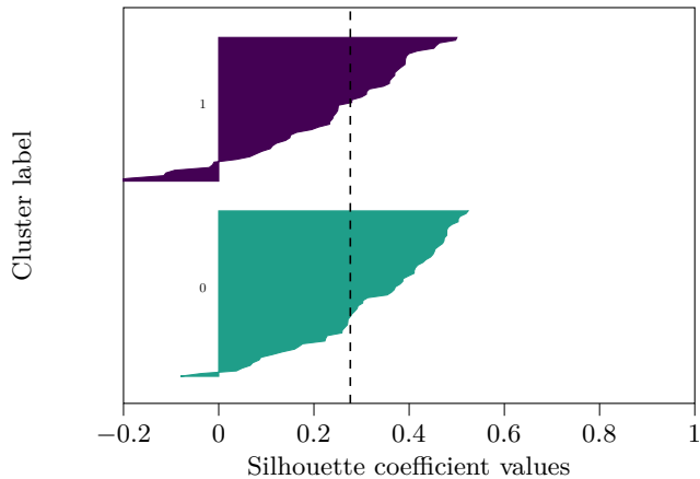
(b) Silhouette coefficient values. The average silhouette score is: 0.276
