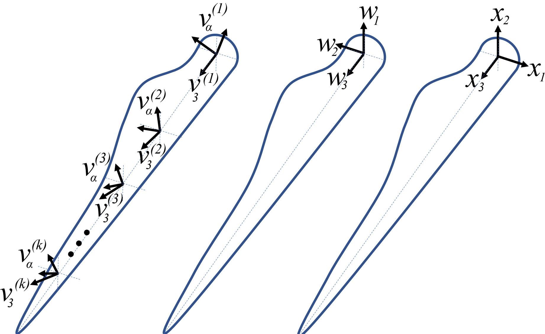
OpenFAST Results Coordinate System
