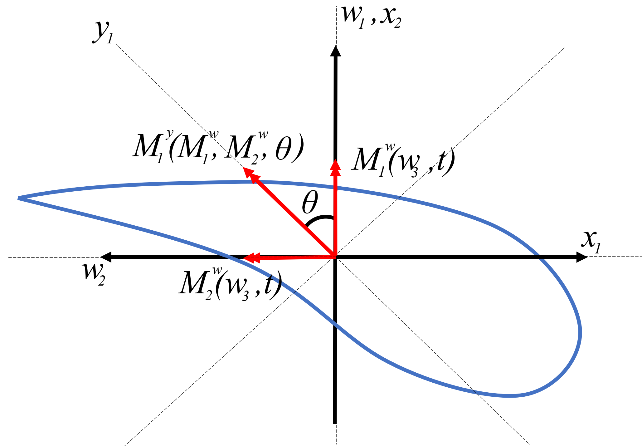
(b) Moment projection axes.
