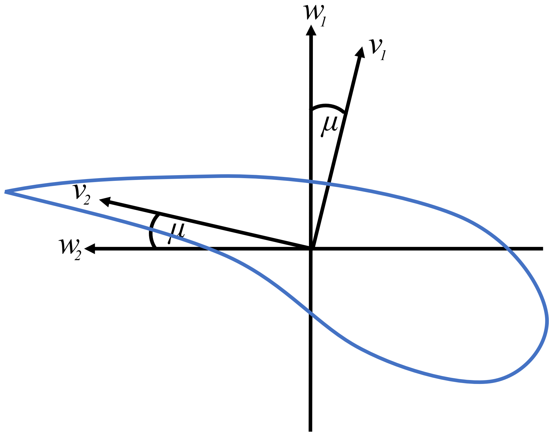
(a) The OpenFAST results are in the v_i coordinate system. The v_i terms are related to the w_i system exclusively with the principal axis angle, \mu .
