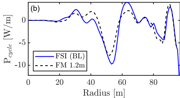
Spanwise flap
