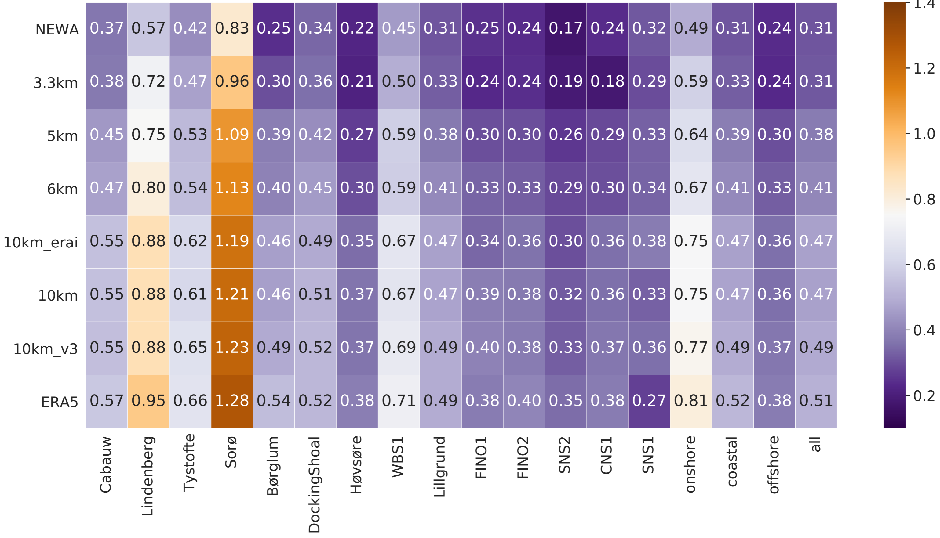
error in ACF(lag1) [ ] \times 10^{-1}
