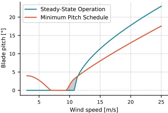
(a) Blade Pitch Schedule
