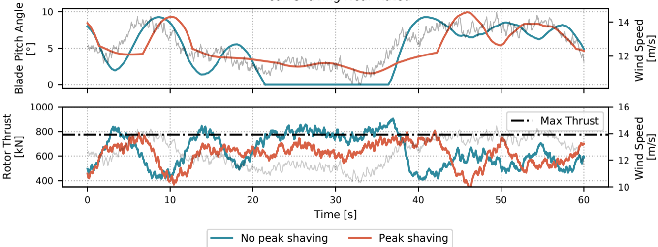
Peak Shaving Near Rated
