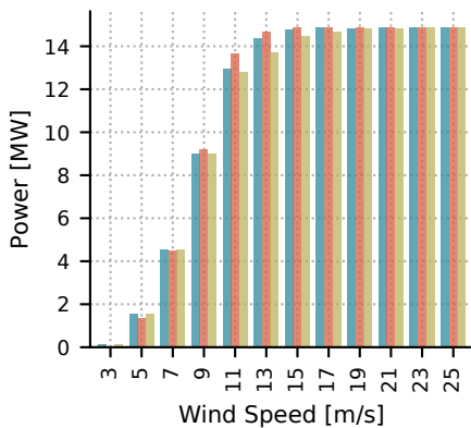
Avg Generator Power (1.1)
