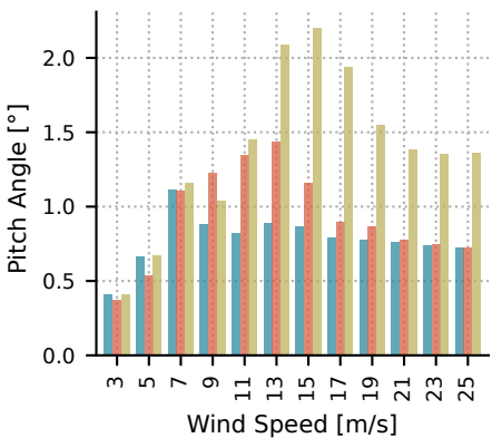
Platform Pitch SD (1.3)
