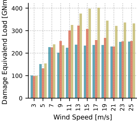
Tower Fore-Aft DEL (1.3)
