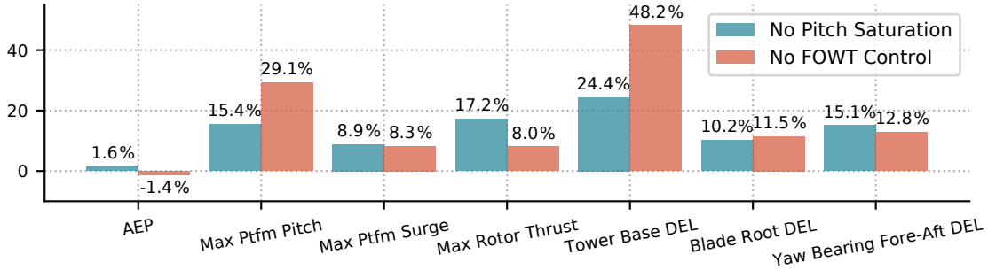
IEA 15-MW AEP and Loads Comparison
