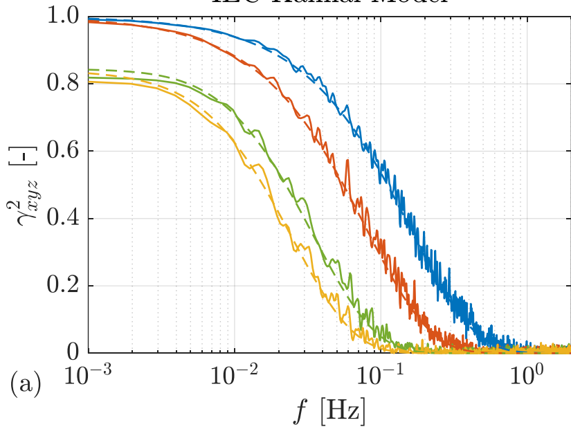
IEC Kaimal Model
