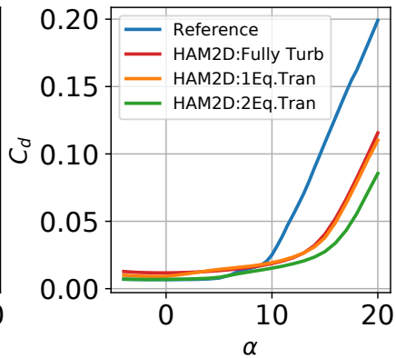
(a) DU91-W2-250 airfoil at Re = 7 \times 10^6
