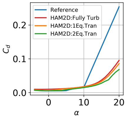
(b) NACA64-618 airfoil at Re = 6 \times 10^6
