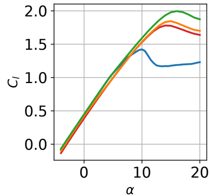
DU91-W2-250
