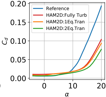
(a) DU93-W-210LM airfoil at Re = 7 \times 10^6
