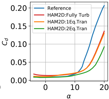
(b) DU97-W-300LM airfoil at Re = 7 \times 10^6
