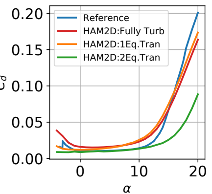
(c) DU99-350 airfoil at Re = 7 \times 10^6
