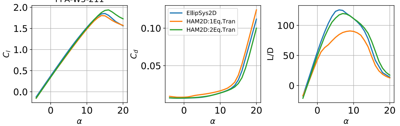
(a) FFA-W3-211 airfoil at Re = 10 \times 10^6
