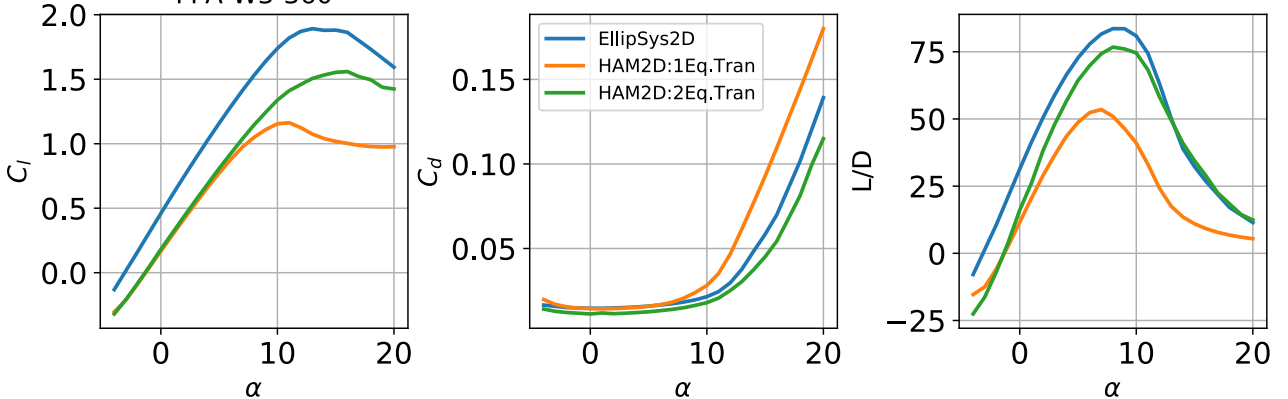
(e) FFA-W3-360 airfoil at Re = 10 \times 10^6
