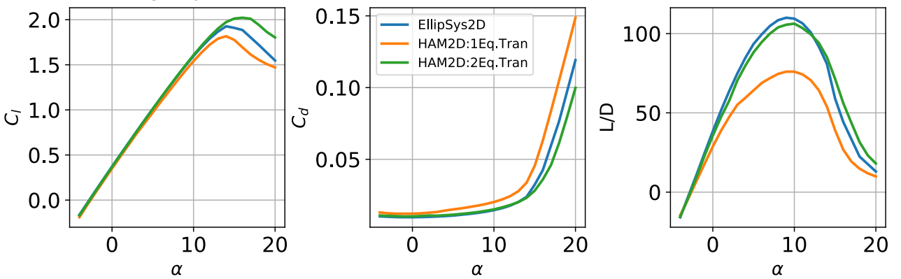
(c) FFA-W3-270BLEND airfoil at Re = 10 \times 10^6
