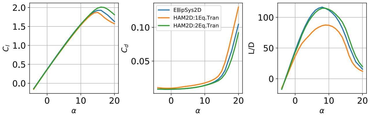
(b) FFA-W3-241 airfoil at Re = 10 \times 10^6
