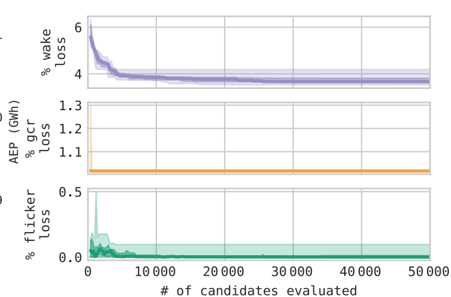
(b) Losses for CMA-ES's solution trajectories
