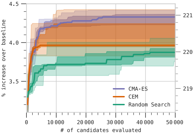
(a) Performance trajectories of current-best solutions
