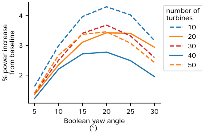
Random turbine layouts
