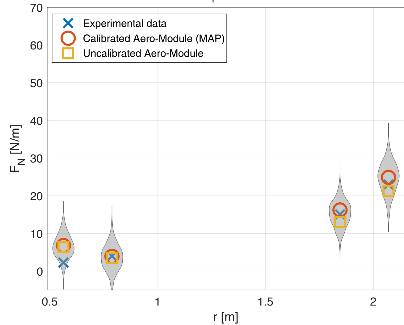
Scenario S_1 (yaw angle 15^\circ )
