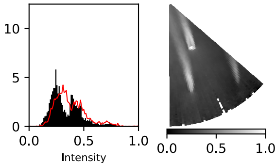
(c) Bimodal
