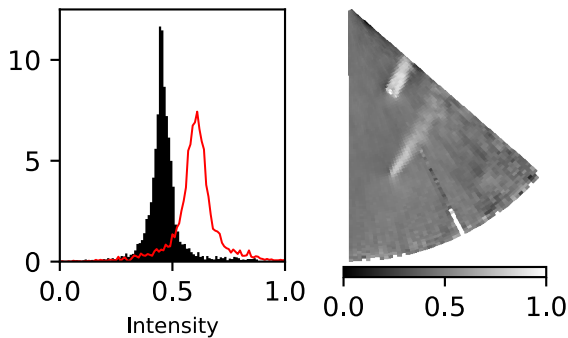
(c) Bimodal
