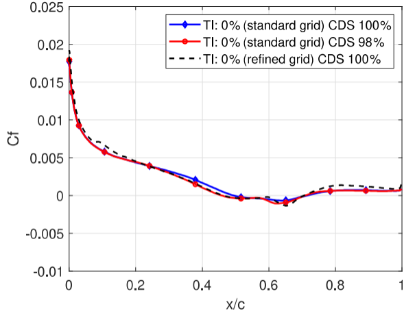
(b) Suction side friction coefficient of the standard vs. the refined grid.
