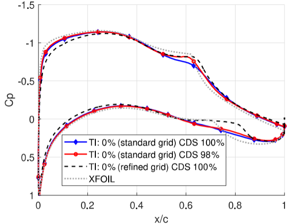
(a) Pressure coefficient of the standard vs. the refined grid. Here, the XFOIL results by Drela (1989) ( N_{crit} = 9 ) are also included.
