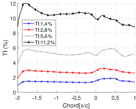
(b) Turbulence intensity development with downstream distance measured at a constant wall-normal distance corresponding to the boundary layer thickness at 50% chord.
