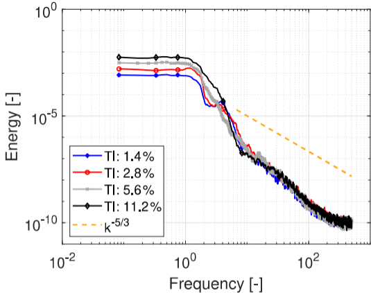
(a) Turbulent kinetic energy spectra of generated inflow turbulence.
